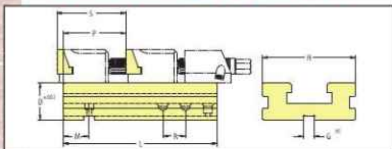
PROLUNGA MOBILE/MOBILE EXTENSION SPE. 81
