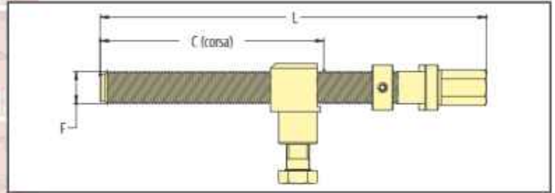
VITE CHIOCCIOLA/SCROLL SCREW PIA 83
