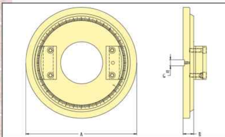
BASE GIREVOLE/ROTATING BASE SPE. 81
