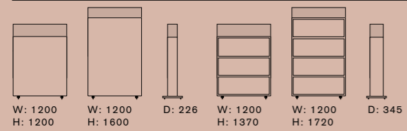
ZORLA Room divider, with & without shelves
